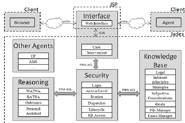
Figure 1: A simplified version of the system architecture.
