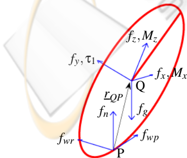
Figure 3: Forces and moments acting on the wheel.
