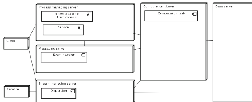
Figure 9: Deployment diagram of KASKADA platform.
