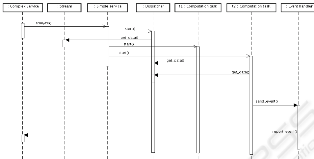
Figure 8: A sequence diagram of the simple service execution within the domain model (see figure 6).
