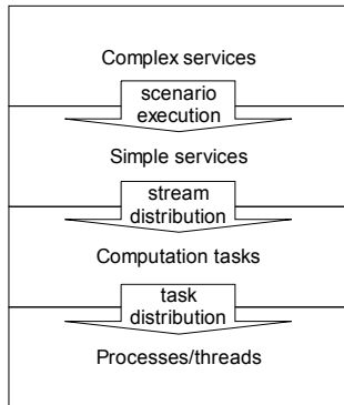
Figure 1: Layered processing model of KASKADA platform.
