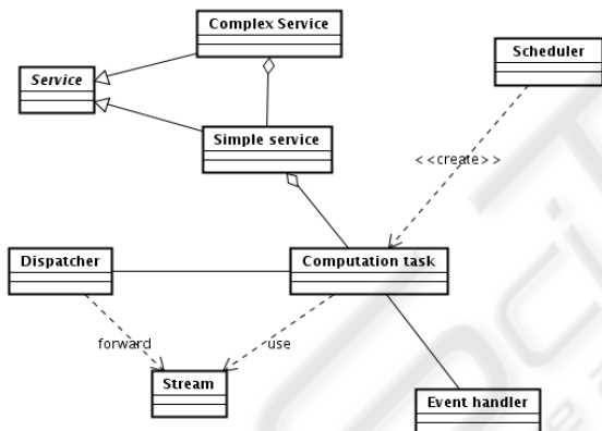
Figure 6: Domain class diagram of the KASKADA platform.
