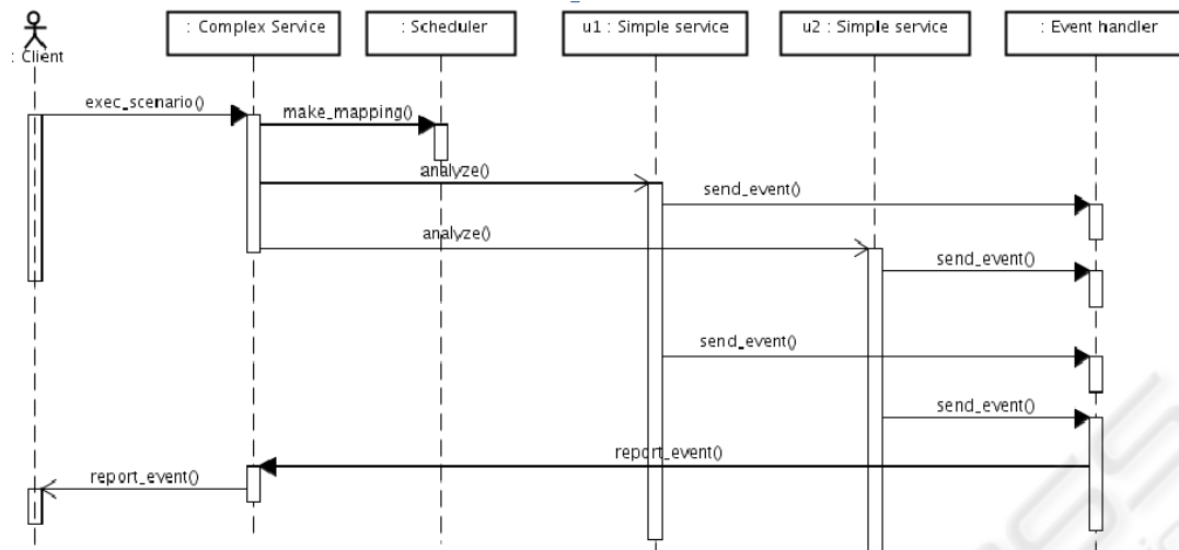
Figure 5: A sequence diagram of the complex service execution within the domain model (see figure 6).
