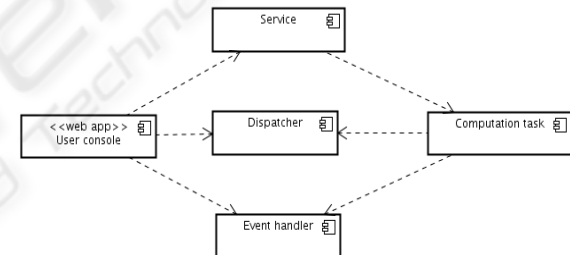
Figure 7: Component diagram of the KASKADA platform.
