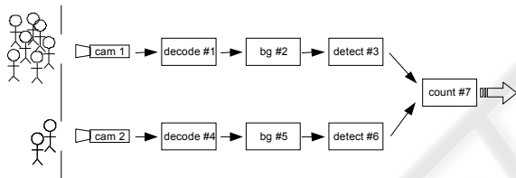
Figure 2: Graph representation of the example scenario.
