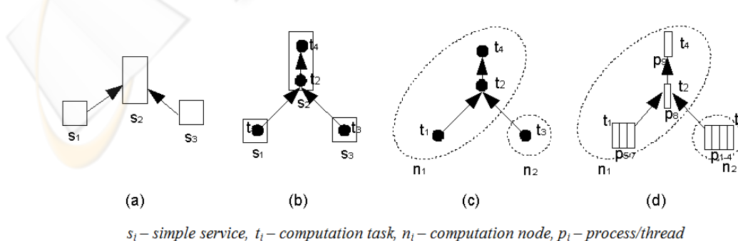
Figure 3: Phases of preparation to service scenario execution: (a) simple services, (b) task graph, (c) graph assignment to the computation nodes, (d) running processes/thread.
