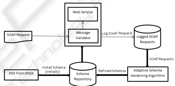
Figure 7: Schematic of Adaptive Schema Hardening Algorithm.
