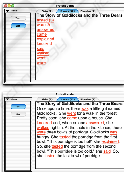
Figure 7: Example of views linked to F_{repE} for PC preterit.
