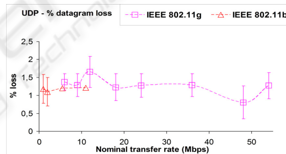
Figure 5: UDP – percentage datagram loss results versus technology and nominal transfer rate.
