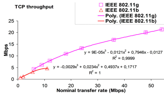
Figure 3: TCP throughput versus technology and nominal transfer rate.
