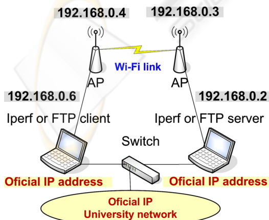
Figure 2: Laboratory setup scheme.
