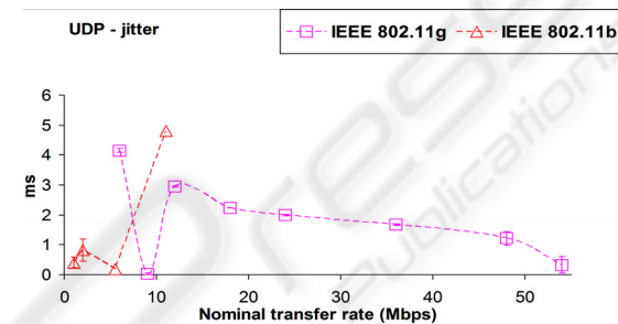
Figure 4: UDP – jitter results versus technology and nominal transfer rate.
