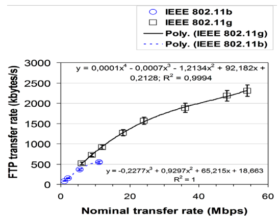
Figure 6: FTP transfer rates versus technology and nominal transfer rate.
