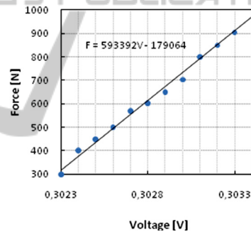
Figure 5: Medial sensor characterization.
