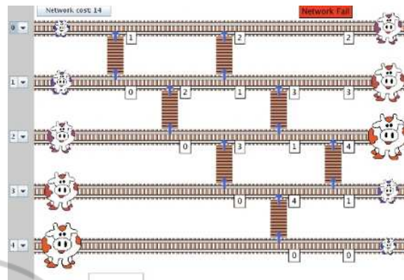
Figure 10: A network that extracts first and second by two applications of the diagonal pattern.
