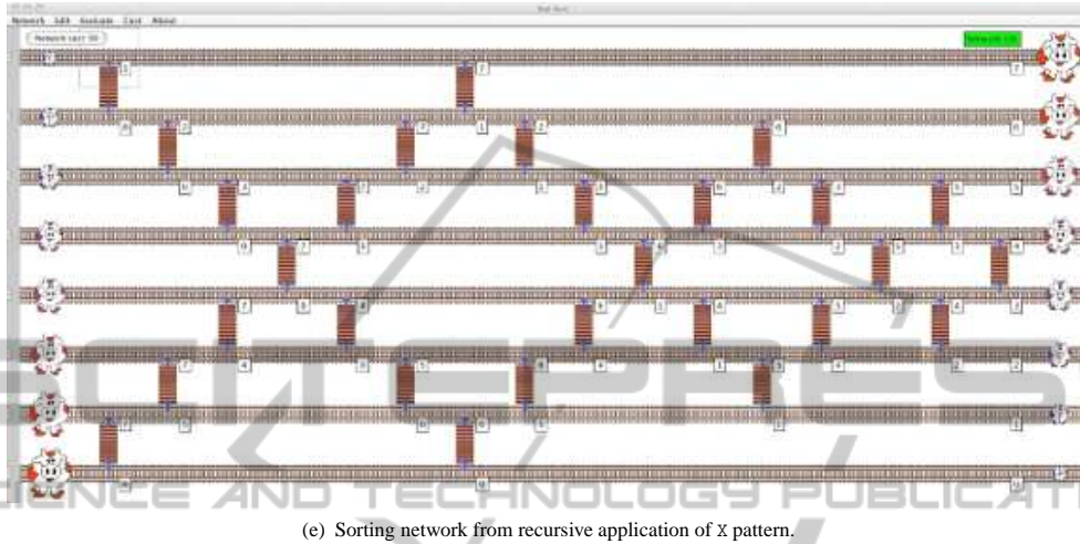
Figure 14: A very symmetrical sorting network by a recursion that finds simultaneously the largest and the smallest item.
