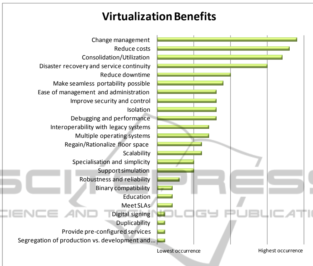
Figure 1: Virtualization benefits.
