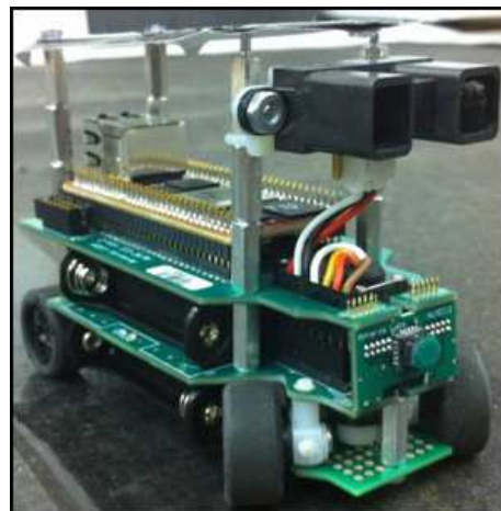
Figure 1: One of the ALMC-100 micro-cars.
