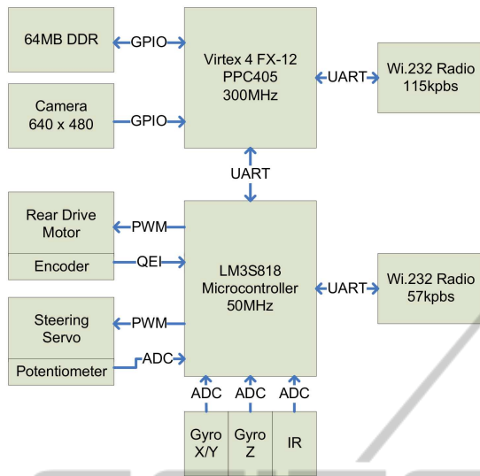
Figure 2: A schematic diagram of the ALMC-100 micro-car hardware.
