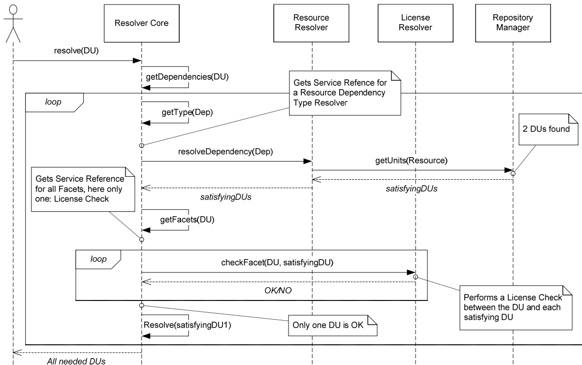
Figure 4: Dependency Resolution.
