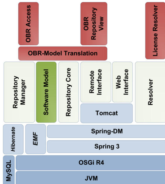
Figure 3: Repository Architecture.
