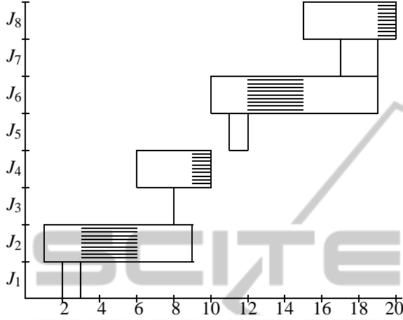
Figure 1: Maximal ranges [l_i, u_i] of possible variations of the processing times p_i, i \in \{2, 4, 6, 8\} , within the stability box S\mathcal{B}(\pi_1, T) are dashed.
