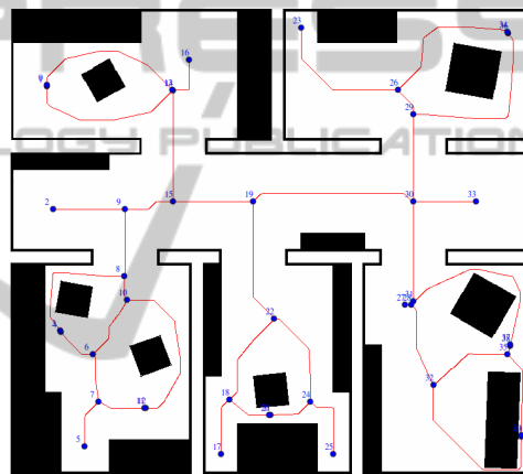
Figure 6: Results for a medium graph (41 vertices) with defined connectivity.
