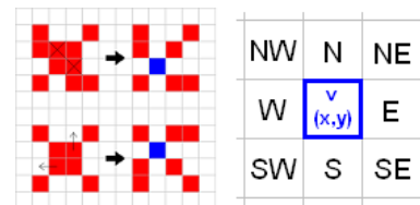
Figure 3: On the left side: Cluster Analysis - Pixel removal on top and pixel shifting below. On the right side: Possible neighbor directions.
