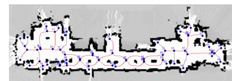
Figure 8: Results for a graph with 70 vertices and a few connectivity constraints.
