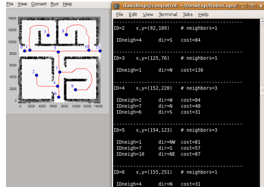
Figure 4: Extracting the graph and relevant topological information. Example of a simple tree-like graph with 12 vertices.
