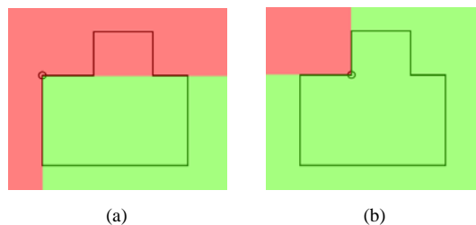
Figure 2: Camera position estimation steps. A convex (a) and a concave (b) corners allow to discard parts of the plane (red).
