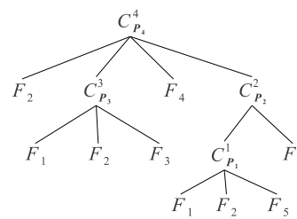
Figure 2: Generic structure of the proposed MNOS model and the existing MNOD. The nodes C_{\mathbf{P}}^n represent the supervised neural models which receive their input directly from leaf nodes F_i and/or other internal nodes C_{\mathbf{P}}^m . In the MNOS model a node C_{\mathbf{P}}^n may use either the sliding window or segments as contextual information to be classified.
