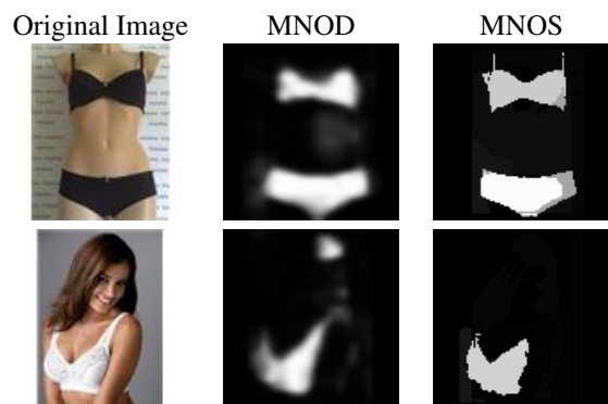
Figure 6: Some examples from the Drezzy dataset of the MNOS's segmentation results using only Sliding Windows (MNOD) and using Sliding Windows and Segments (MNOS).
