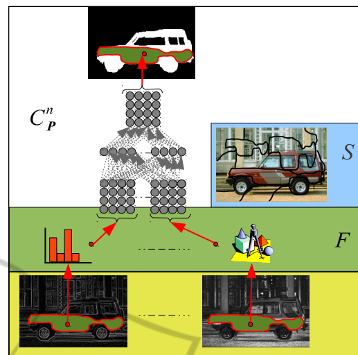
Figure 4: Generic structure of a MNOS node C_P^n . It generate the set of segments S = \{S_1, \dots, S_N\} on the original scaled image. Then, for each input image from child nodes and for each segment it calculate the features F = F_I \cup F_S and compose the patterns for the neural network. Finally, the neural model prediction values are used to shape the output image of the node C_P^n .
