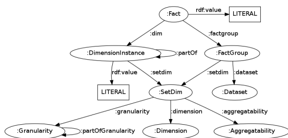
Figure 2: RDF-schema to store multidimensional data.
