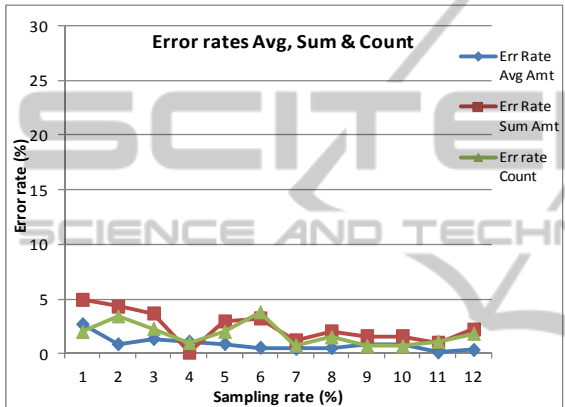
(c) Error rates for query with condition on two dimensions (medium relevancy ratio).
