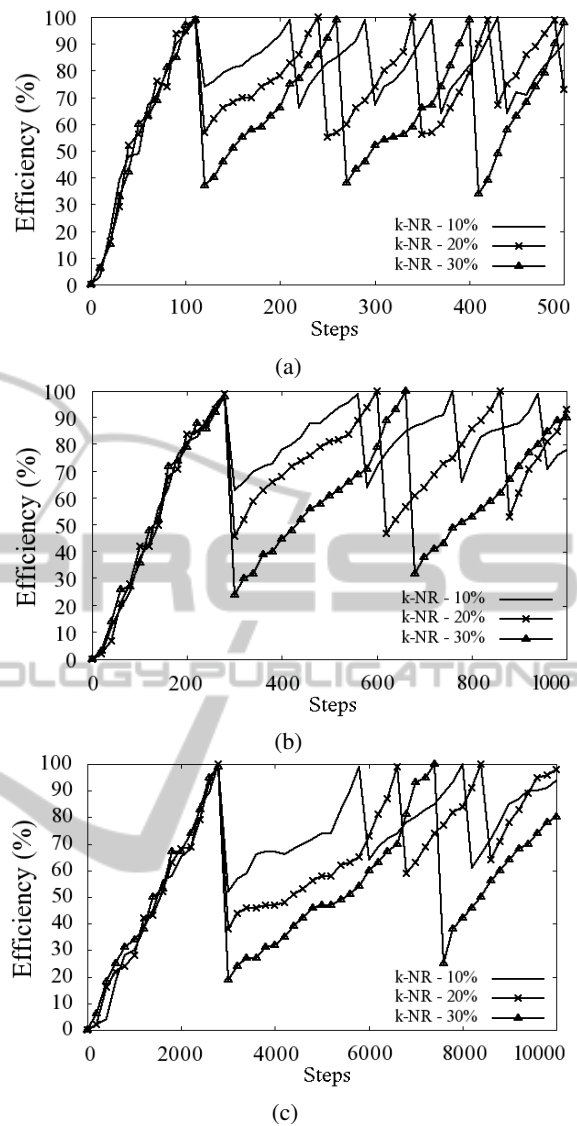
Figure 5: Agent adaptation using the k -NR in a: (a) 16-state environment, (b) 25-state environment, (c) 64-state environment.
