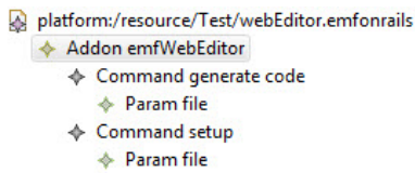
Figure 5: Add-on model of the EMF web editor. This model is an instance of the meta-model shown in Figure 3.
