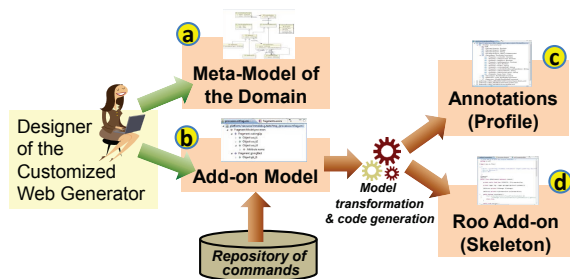
Figure 2: Step 1: Building a customized web generator.
