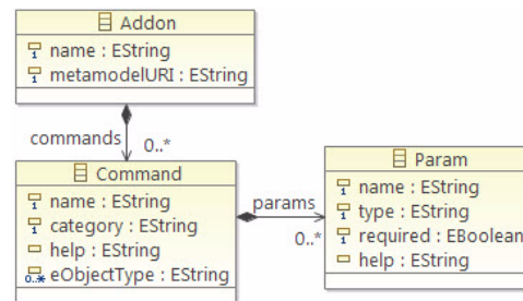
Figure 3: Meta-model for Spring Roo add-ons.
