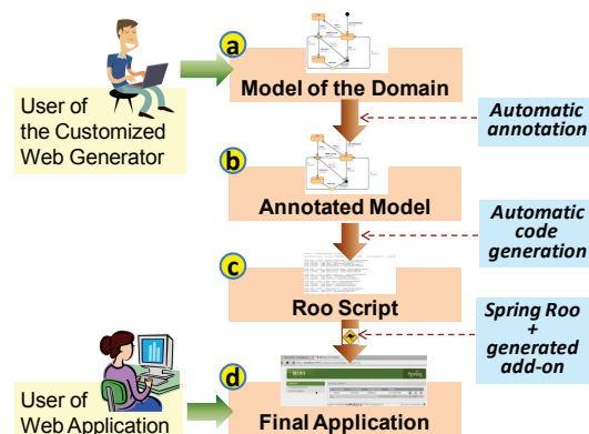
Figure 4: Step 2: Using the customized web generator to synthesize the final web application.
