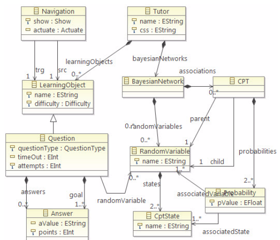
Figure 7: Most significant elements in the tutor model.
