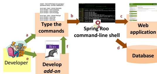
Figure 1: Web application development with Spring Roo.
