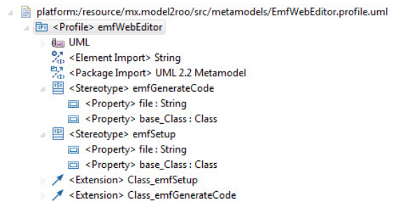
Figure 6: Annotations from the EMF web editor.
