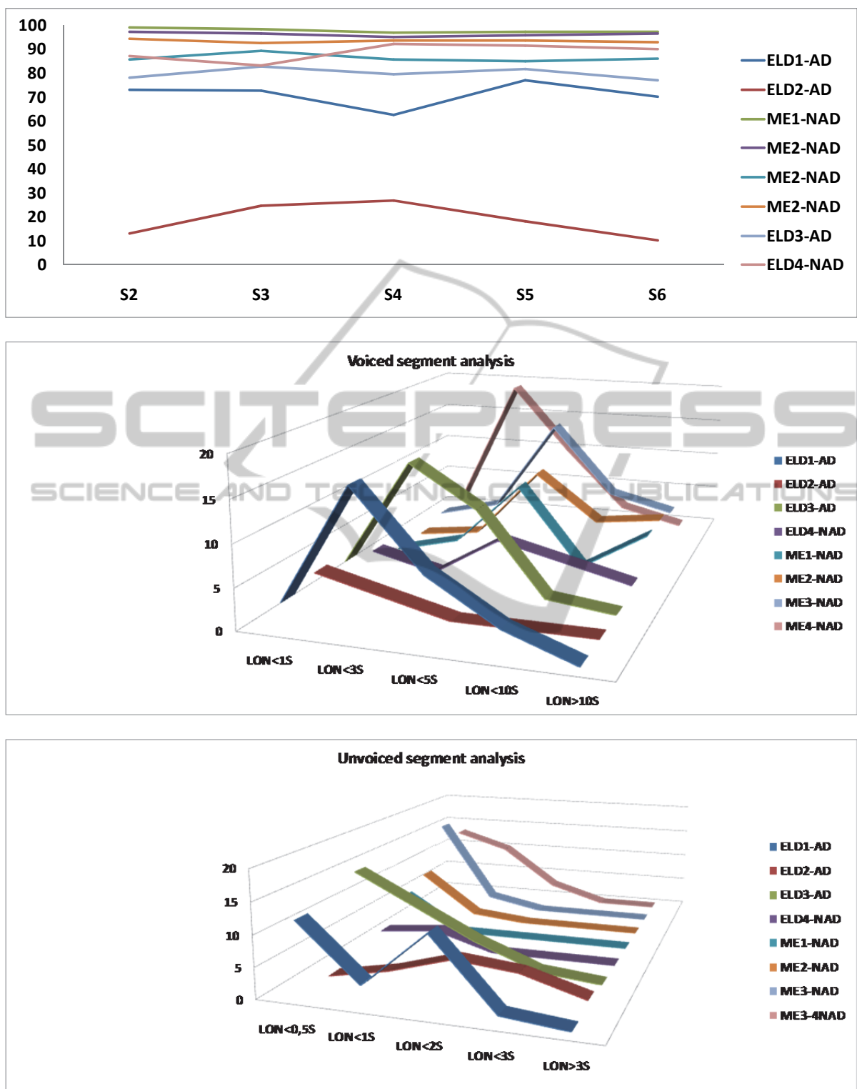
Figure 7: (a) The Spontaneous Speech Evolution with regard to the Speech Percentage along the time, for the consecutive segments (S2:S6). (b) Voiced segment analysis with the regard to segment length (c) Unvoiced segment analysis with the regard to segment length.
