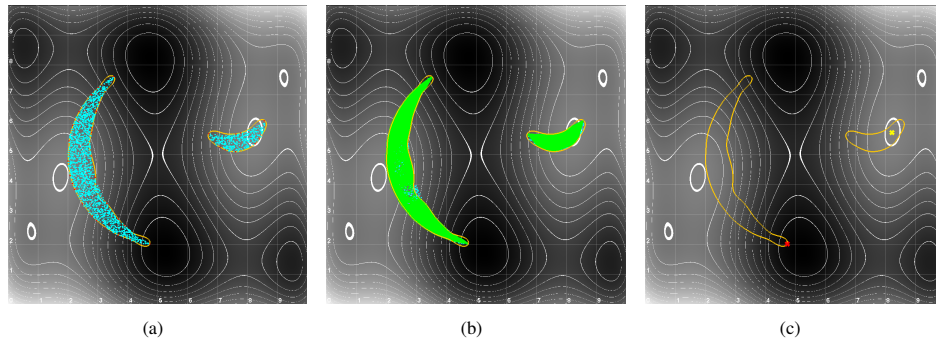
Figure 1: 1(a): Sample from a artificial double banana shaped region. 1(b): Re-sampling the feasible region by mapping random points from [0, 1]^2 . 1(c): marked optima of the Six-hump camel back objective function withing the used domain.
