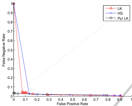
Figure 4: Curve for Pyramid Lucas-Kanade, Lucas-Kanade and Horn-Schunck at 20 histogram bins and region size of 16 x 16. Test dataset: Directional.
