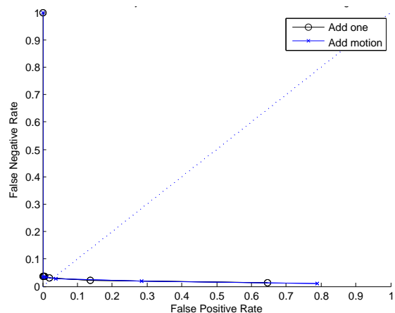
Figure 8: Frame level abnormality detection on the directional dataset, with the two different updating methods.
