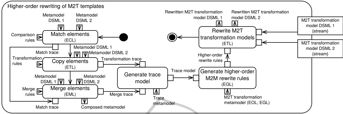
Figure 7: Process of higher-order rewriting of M2T templates.
