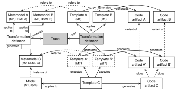
Figure 4: M2T template rewriting for DSML integration.
