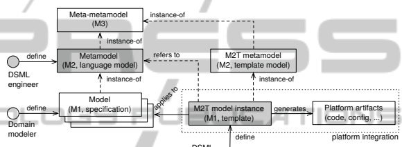
Figure 2: M2T template models.
