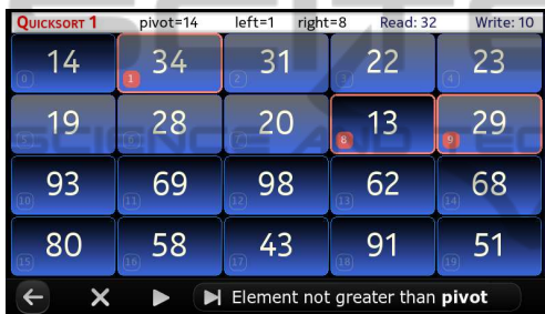
Figure 5: Prototest application in landscape mode.
