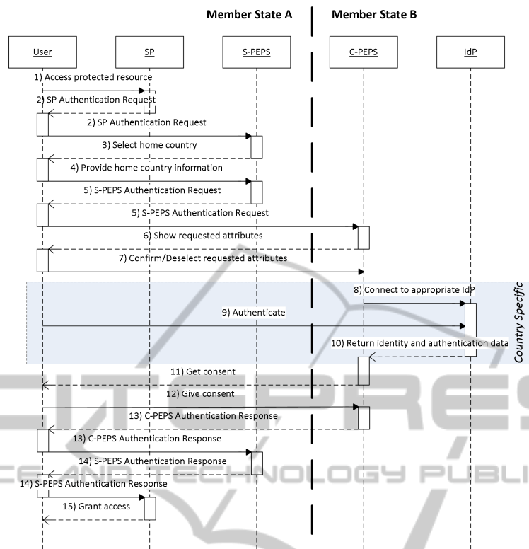
Figure 2: The PEPS-PEPS Process Flow.
