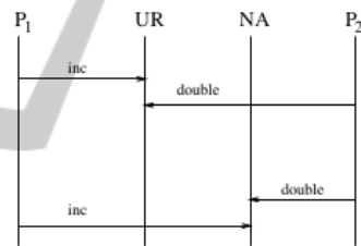
Figure 3: An implied bad scenario in Alur’s plant (Alur et al., 2003) (hidden by Wright’s glue specification).
