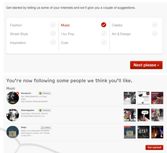
Figure 7: Welcome workflow.
