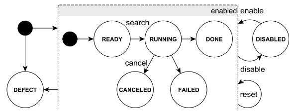
Figure 5: Search States.
