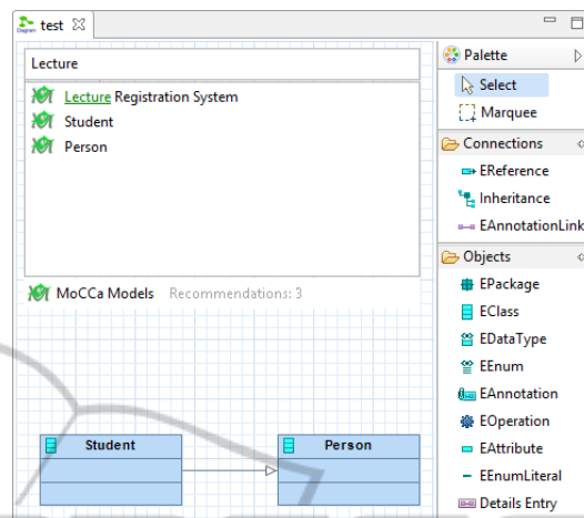
Figure 8: Simulation UI.
