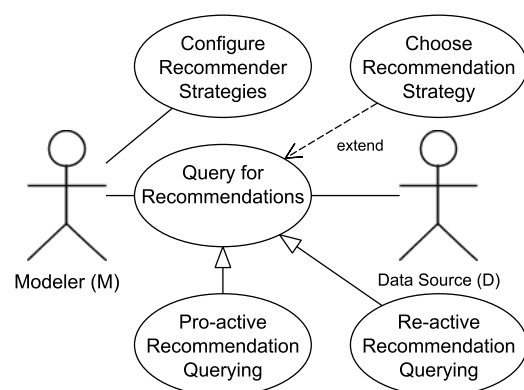
Figure 1: Model Recommender Framework Use Cases.
