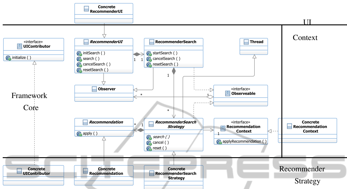
Figure 3: Coarse Grain Architecture.
