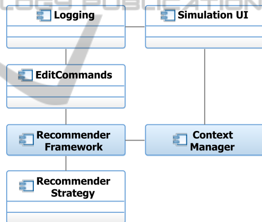
Figure 7: Simulation Architecture.
