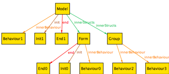
Figure 3: Instance of the Alloy model (from Figure 2) regarding PARADIGM hierarchical levels.
