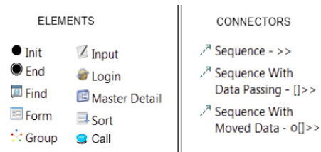
Figure 6: PARADIGM’ Syntax.
