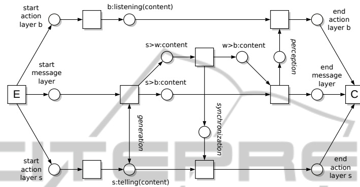
Figure 6: Communication pattern.
