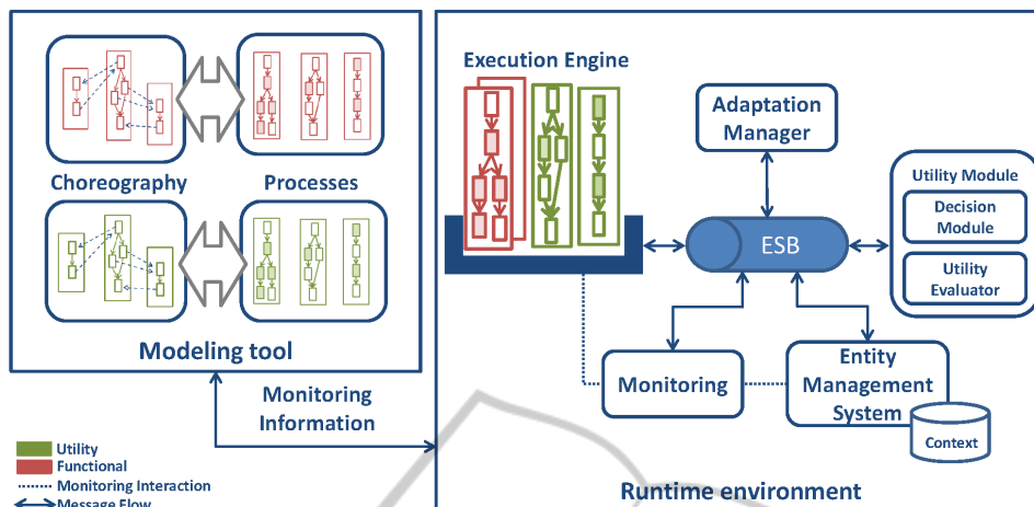
Figure 3: Architecture overview
