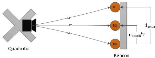
Figure 6: Topography of quadrotor orthogonal to reference beacon.
