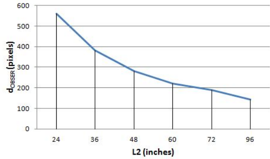
Figure 7: L2 vs d_{observed} when characterizing Wii camera.
