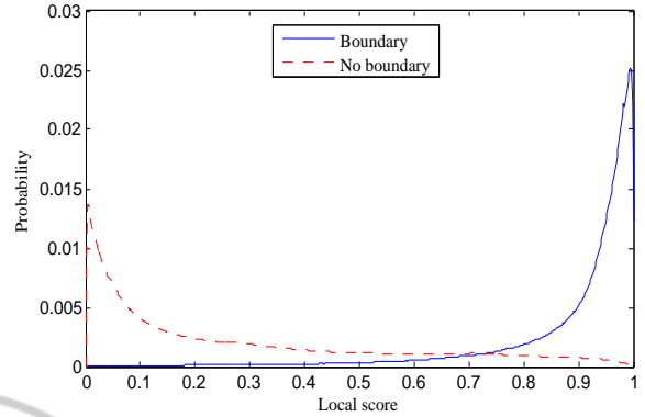
Figure 2: Probability distribution of MLP-based local score values at, and away from, phoneme boundaries, estimated from TIMIT.
