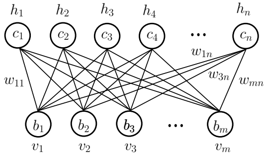
Figure 1: A restricted Boltzmann machine (RBM).
