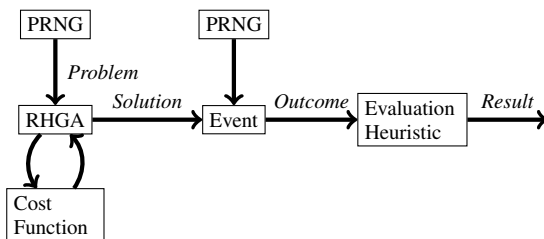
Figure 3: Simulation model. A pseudo-random number generator (PRNG) generates simulation scenarios in which the RHGA uses some cost function Cost 1 to determine a solution (where tugs should move). The PRNG then generates an event of drift, which depending on the current position of the tugs may be critical or not. The outcome (saving or not saving the drifting ship) is then quantified as Cost 2 by an evaluation heuristic.
