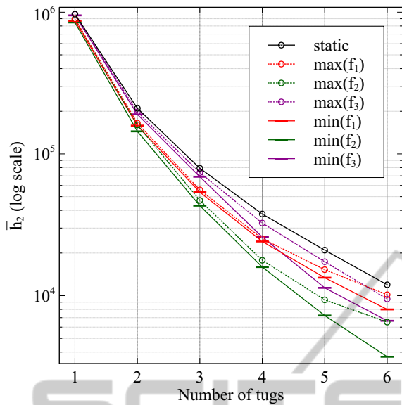
Figure 6: Maximum and minimum mean h_2 evaluated for 1–6 tugs and cost functions f_1 – f_3 and the static strategy.
