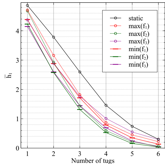
Figure 4: Maximum and minimum mean h_1 evaluated for 1–6 tugs and cost functions f_1-f_3 and the static strategy.
