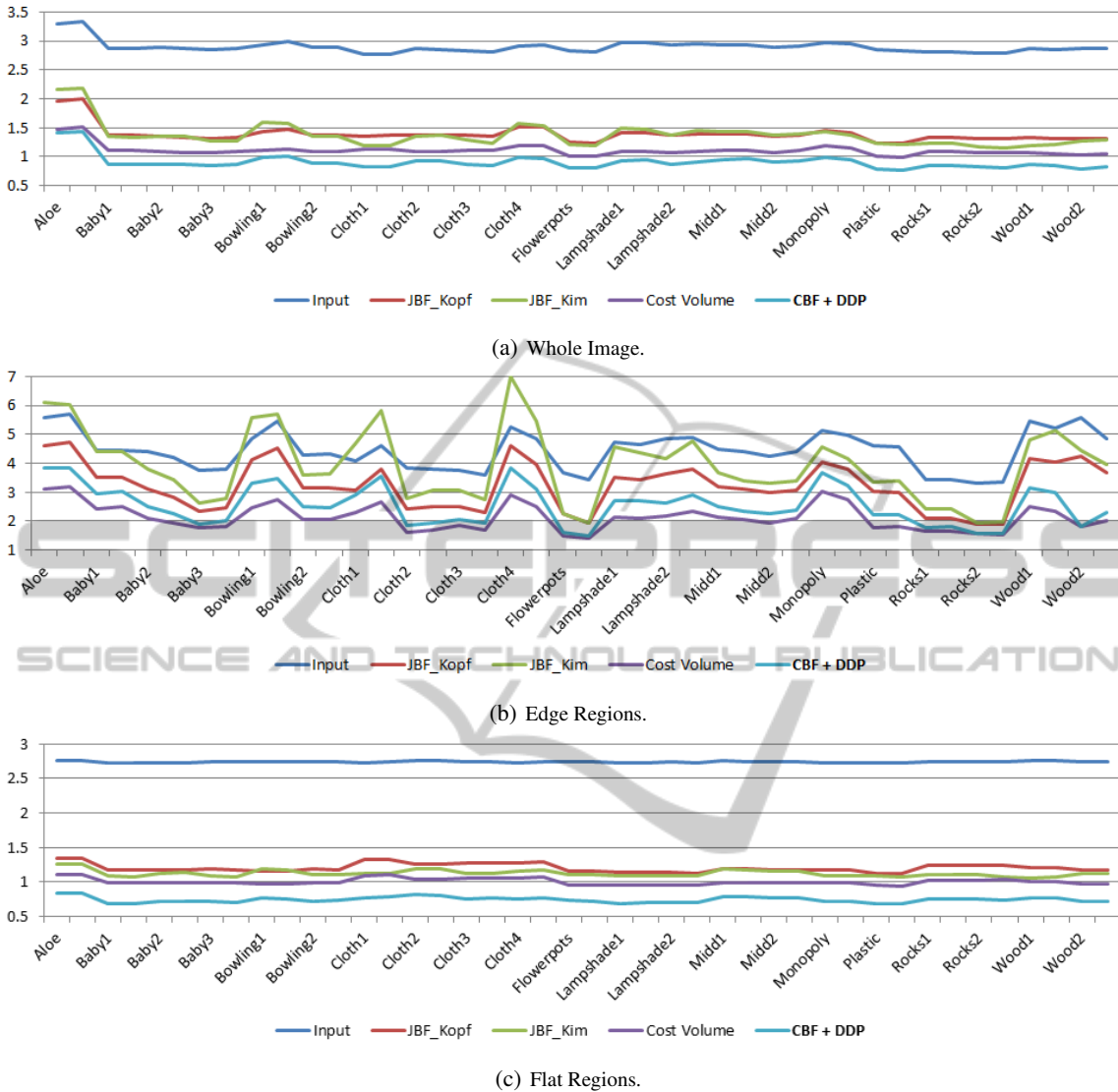
Figure 6: Mean Error (see Equation 7) for all datasets of (Scharstein and Szeliski, 2003) in denoted regions.
