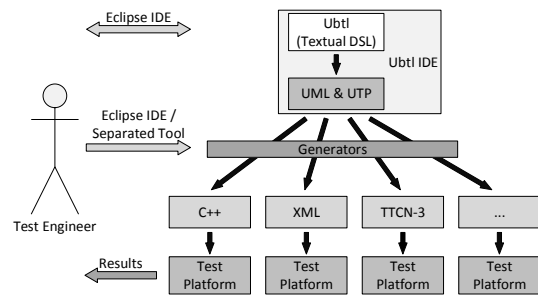
Figure 1: UbtI application number one shows how a test engineer could use the UbtI IDE and different code generators.
