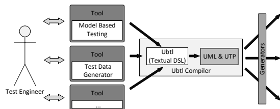
Figure 2: UbtI application number 2 illustrates how UbtI could be leveraged by other tools.
