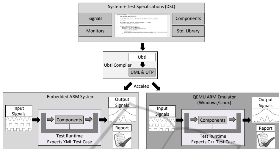
Figure 6: Test workflow used to evaluate Ubt1: (a) test specification in Ubt1, (b) Ubt1 compilation and generation of concrete test cases, and (c) test execution on ARM embedded system (left) or ARM QEMU emulator (right).
