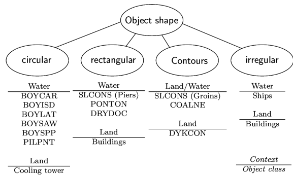
Figure 6: Sorting of S-57 object classes (selection) by shape (geometry type) and context.
