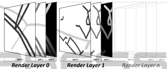
Figure 8: Exemplary render-to-texture configuration for multiple segment categories. Each render layer comprises three render targets (width distance field, respective length distance-field, and linear fragment depth).
