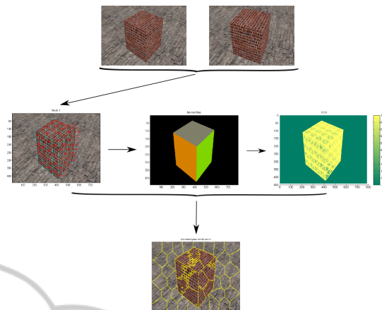
Figure 3: Framework of our proposed over-segmentation method using scene geometry. At the top, the two images I and I' . In the second row: the Delaunay triangulation from 2D interest points matched with the other view; the normal map estimated on the faces of the mesh and the similarity map between both views. The over-segmentation results is coherent with the scene geometry.
