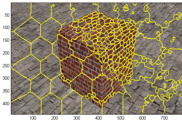
Figure 2: K-means superpixels compactness comparison with a small number (50) of desirable superpixels: bottom-left hard compactness at m = 40 and top-right a soft compactness at m = 5 .
