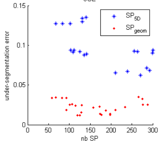
Figure 7: Boundary recall and undersegmentation error for SP_{5D} based on SLIC and the proposed approach SP_{geom} .
