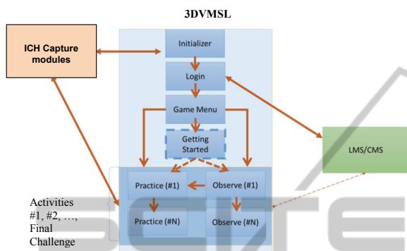
Figure 1: Detailed System Architecture of Game-like Applications.
