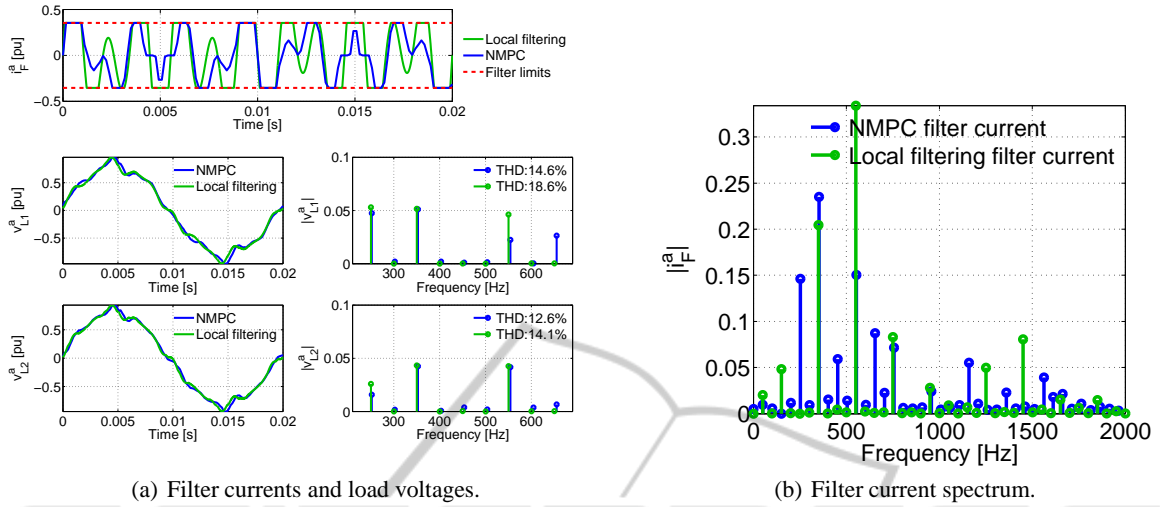
Figure 5: Case 2 (asymmetric loads): Filter currents and filtered load voltages.
