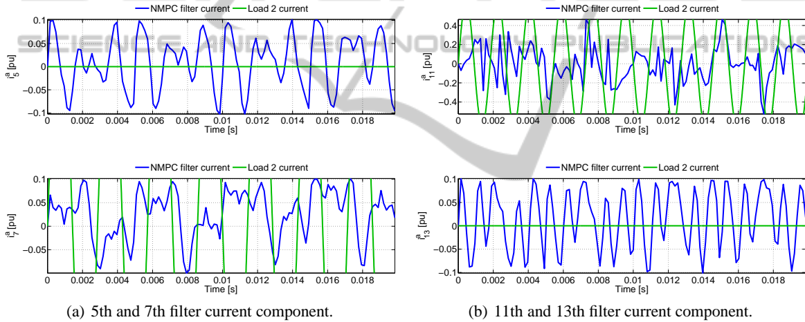
Figure 6: Case 2 (asymmetric loads): Filter current components.
