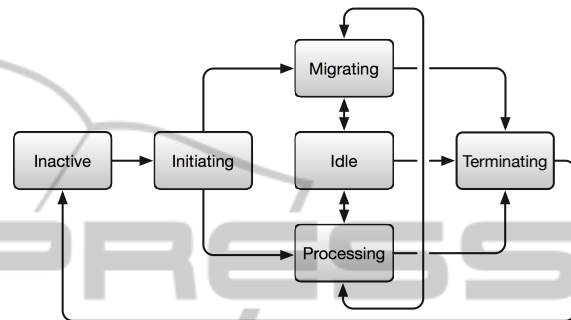
Figure 4: Transitions between Virtual Machine states.
