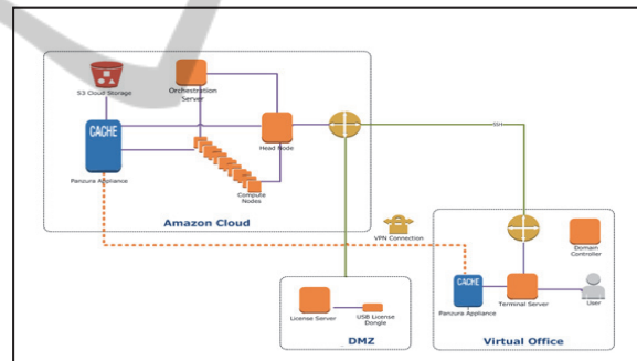
Figure 1: Conceptual Design.
