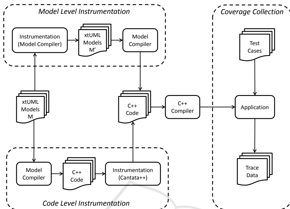
Figure 4: The setup for measuring test coverage.
