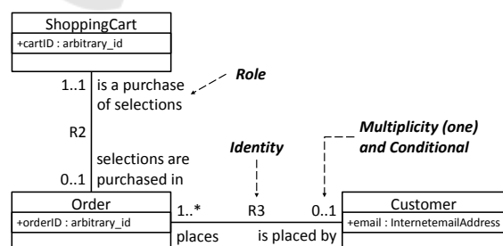
Figure 1: Part of the Online Bookstore Domain class diagram.(Mellor and Balcer, 2002).
