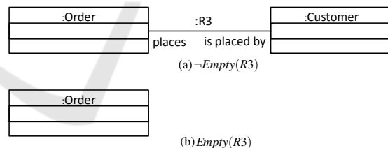
Figure 2: Valid configurations of instances in some point in time.
