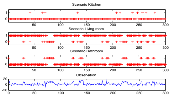
Figure 2: Hidden Markov Model: hidden state and observation.
