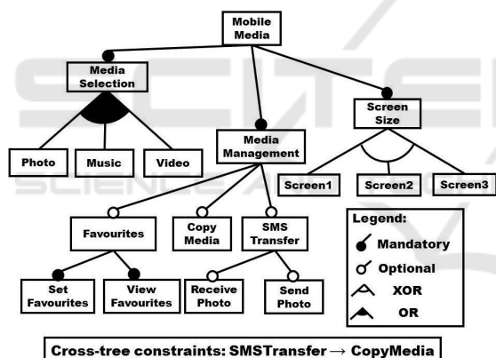
Figure 2: MobileMedia Feature Model.
