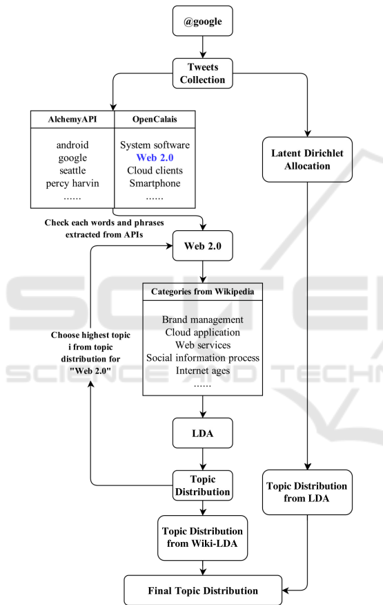
Figure 4: Overall prediction process for test user @google.
