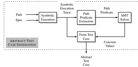
Figure 3: Abstract test case generation using Symbolic execution.
