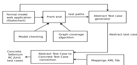
Figure 1: Proposed Test Generation Method used by our ACT tool.
