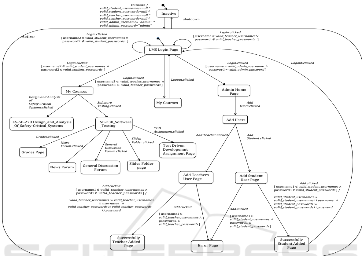
Figure 2: Formal Model showing Web Navigation of Learning Management System using UML State chart model.
