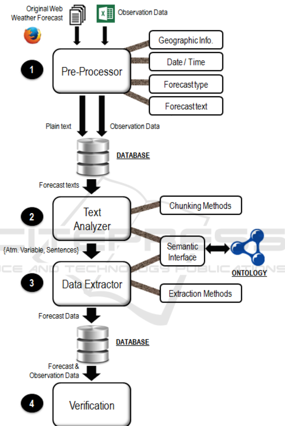
Figure 3: Stages of AEMIX system to extract numerical data from weather forecasts on the Web. The system aims at verifying them, by using patterns embedded in an ontology that drives the extraction process.
