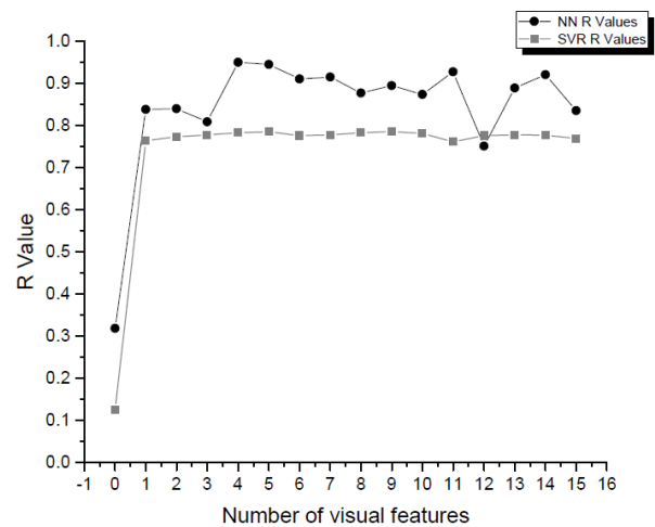
Figure 7: The relationship between the number of features and the R-Value in the NN model and the SVR model.
